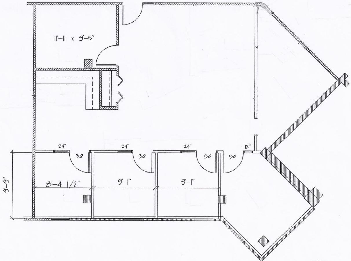
PRELIMINARY FLOOR PLAN - SUITE 1040 SCALE: 1/8" = 1'-0"
